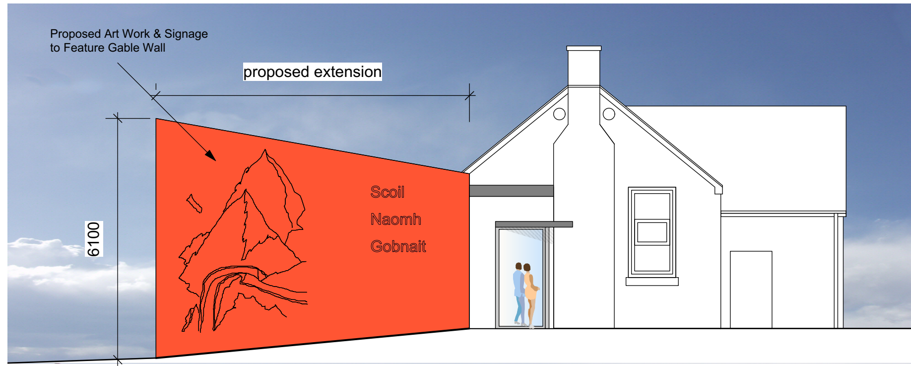
PROPOSED SIDE ELEVATION SCALE 1:100 @ A3
