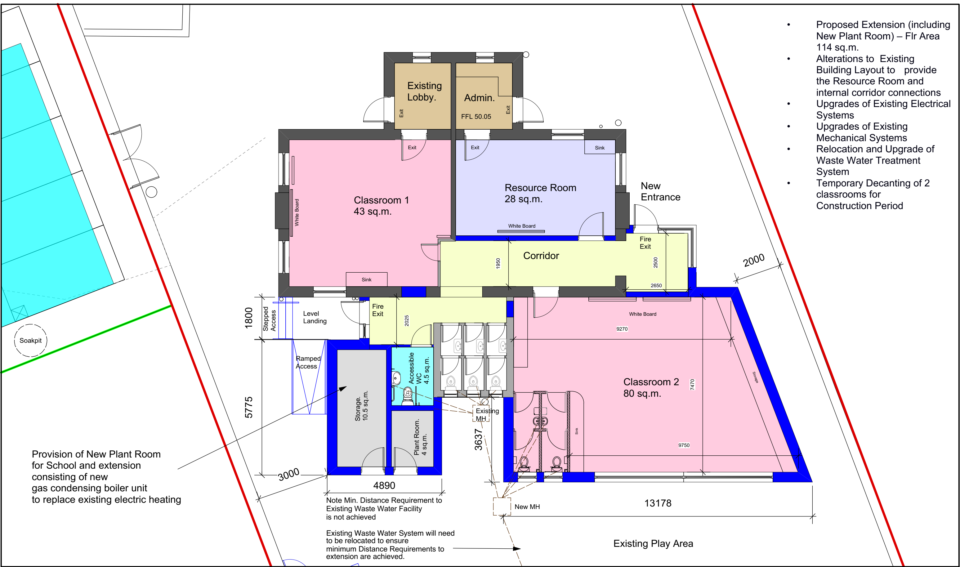
Ground Floor Plan showing Proposed Extension Scale 1:100 at A3
